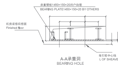
A-A 承重洞 BEARING HOLE
