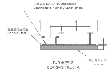
B-B 承重墩 BEARING FRUSTA
